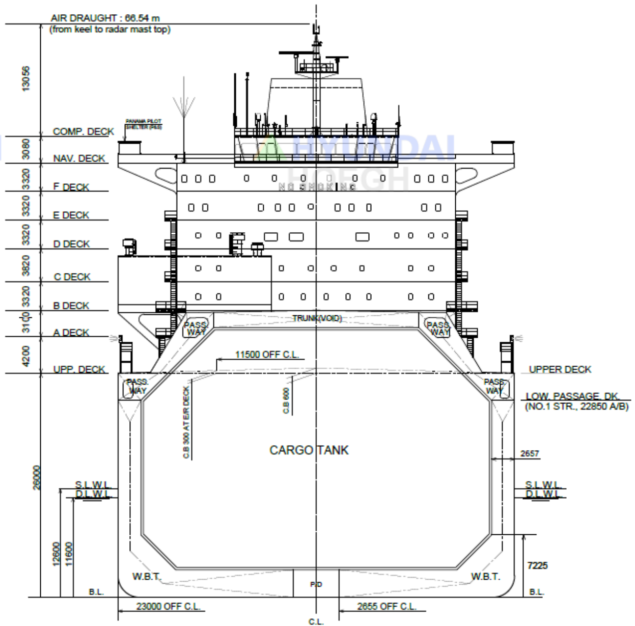
MIDSHIP SECTION
